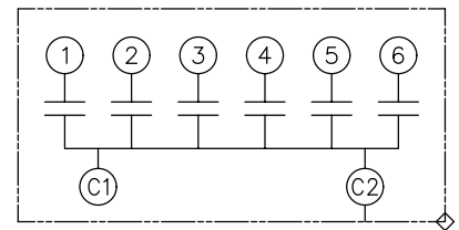
SCHMATIC DIAGRAM - 601
