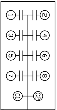
SCHEMATIC DIAGRAM - 801
