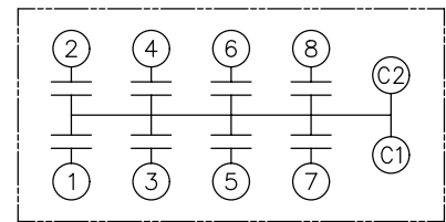
SCHEMATIC DIAGRAM - 800
