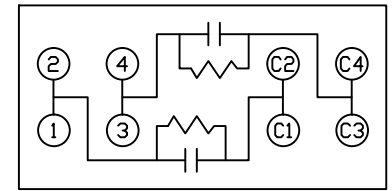
SCHEMATIC DIAGRAM - 240
