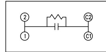
SCHEMATIC DIAGRAM - 107
