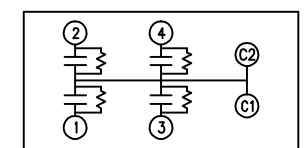
SCHEMATIC DIAGRAM - 422
