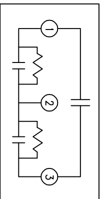
SCHEMATIC DIAGRAM - 304
