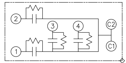
SCHEMATIC DIAGRAM - 432
