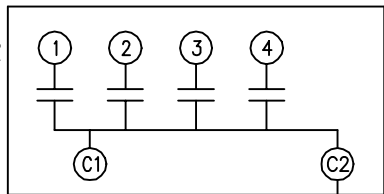
SCHEMATIC DIAGRAM - 436
