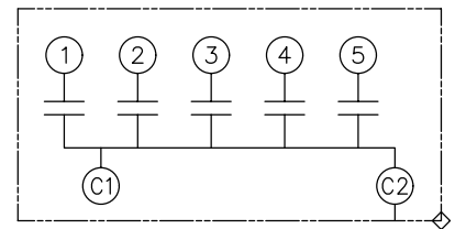
SCHEMATIC DIAGRAM - 506
