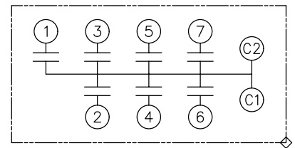
SCHEMATIC DIAGRAM - 705
