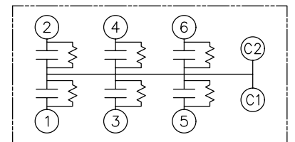
SCHEMATIC DIAGRAM - 617
