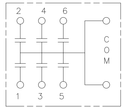
SCHEMATIC DIAGRAM
