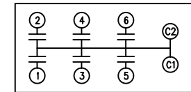
SCHEMATIC DIAGRAM - 615
