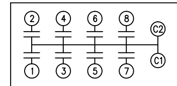
SCHEMATIC DIAGRAM - 800
