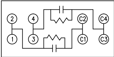
SCHMATIC DIAGRAM - 240
