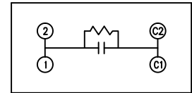
SCHMATIC DIAGRAM - 107
