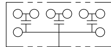
SCHMATIC DIAGRAM
