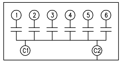
SCHEMATIC DIAGRAM - 601
