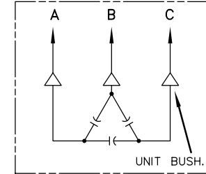
SCHMATIC DIAGRAM INCLUDES DISCHARGE RESISTORS
