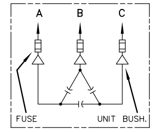
SCHMATIC DIAGRAM
