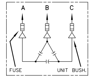
SCHMATIC DIAGRAM INCLUDES DISCHARGE RESISTORS
