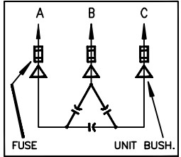
SCHMATIC DIAGRAM
