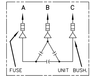
SCHEMATIC DIAGRAM INCLUDES DISCHARGE RESISTORS
