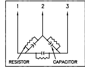
SCHMATIC DIAGRAM - 302
