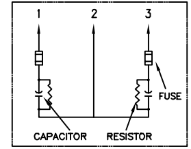
SCHEMATIC DIAGRAM - 227
