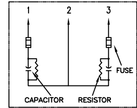
SCHEMATIC DIAGRAM - 227
