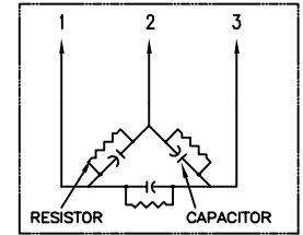
SCHMATIC DIAGRAM - 302
