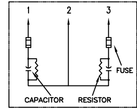
SCHMATIC DIAGRAM - 227
