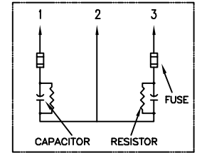
SCHMATIC DIAGRAM - 227
