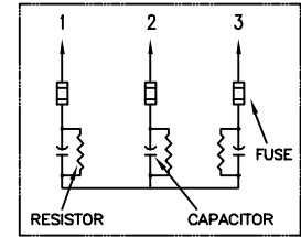
SCHEMATIC DIAGRAM - 337
