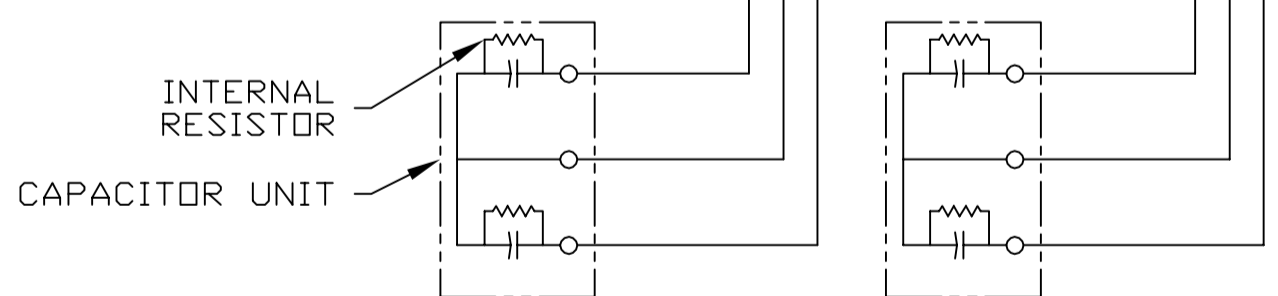
CONNECTION DIAGRAM
