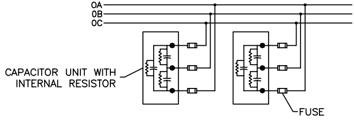
CONNECTION DIAGRAM
