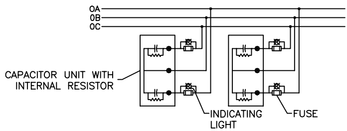
CONNECTION DIAGRAM
