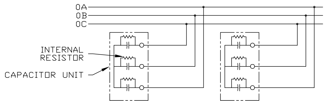
CONNECTION DIAGRAM
