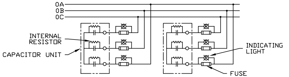
CONNECTION DIAGRAM
