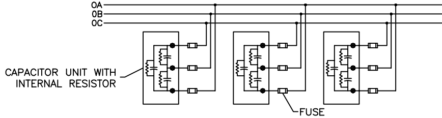
CONNECTION DIAGRAM
