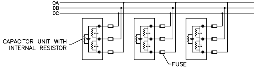
CONNECTION DIAGRAM
