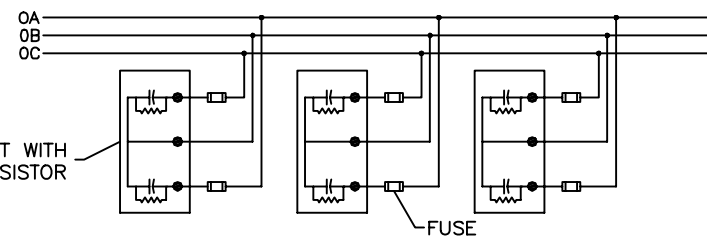
CONNECTION DIAGRAM
