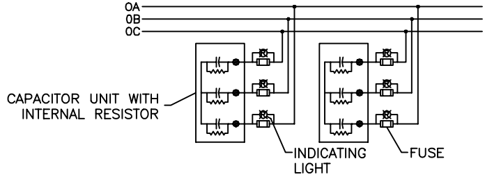
CONNECTION DIAGRAM
