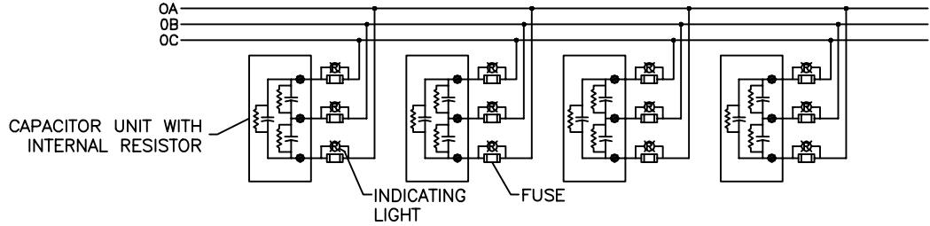
CONNECTION DIAGRAM
