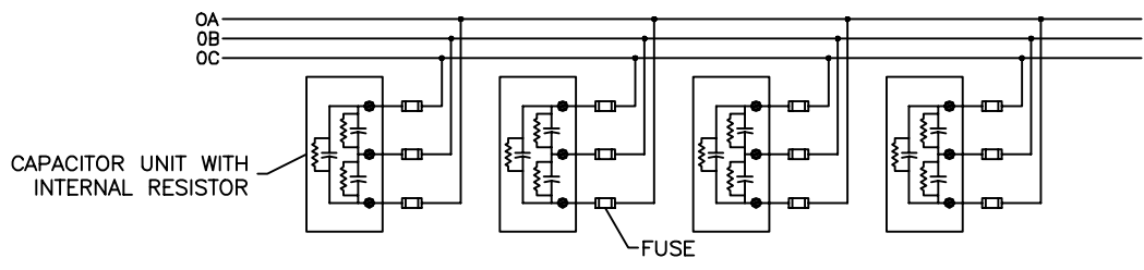
CONNECTION DIAGRAM
