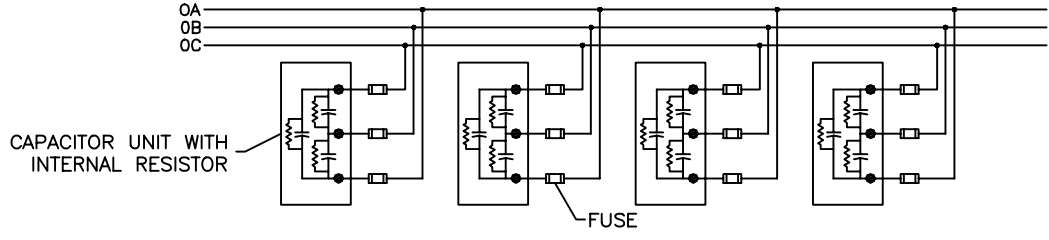
CONNECTION DIAGRAM
