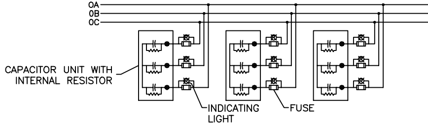
CONNECTION DIAGRAM
