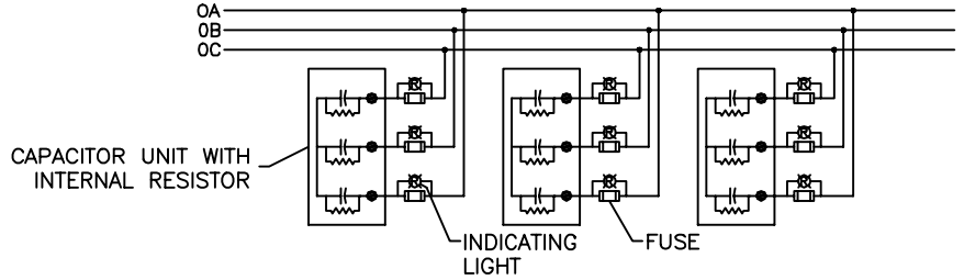
CONNECTION DIAGRAM
