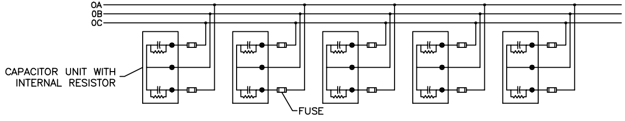
CONNECTION DIAGRAM
