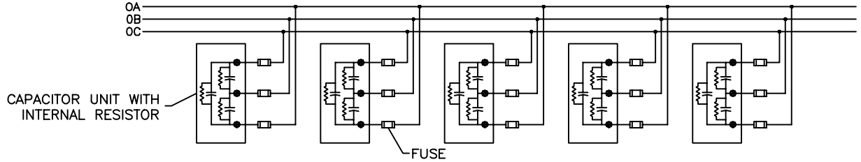
CONNECTION DIAGRAM
