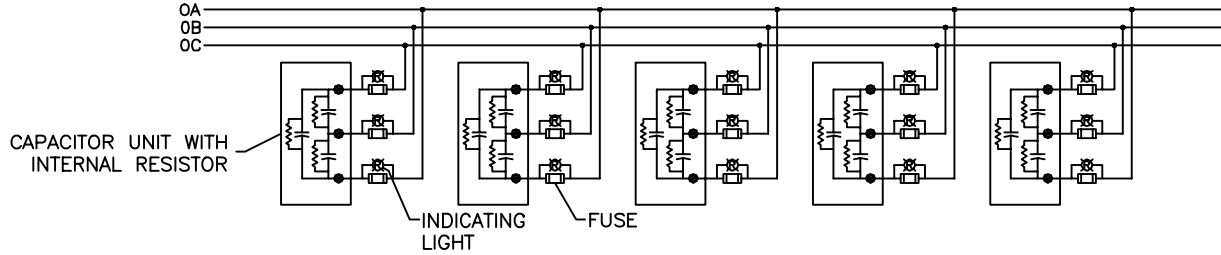
CONNECTION DIAGRAM
