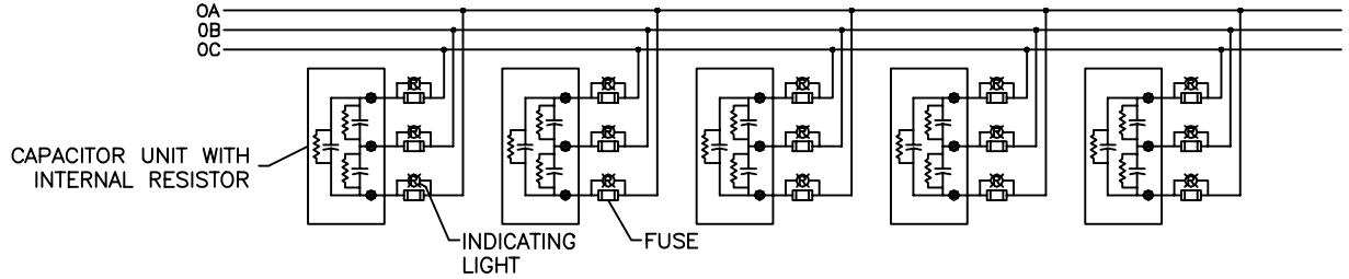
CONNECTION DIAGRAM
