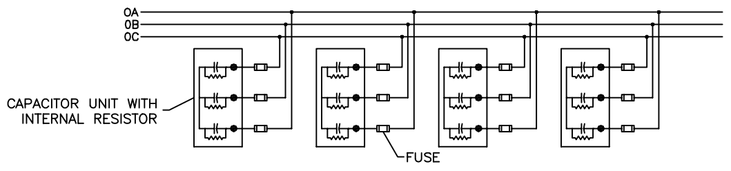
CONNECTION DIAGRAM
